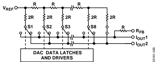
Figure 29. Simplified Ladder
